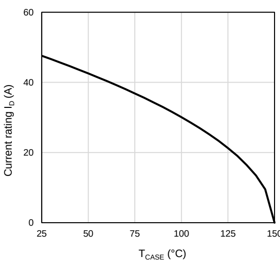
Figure 12: Current De-rating
